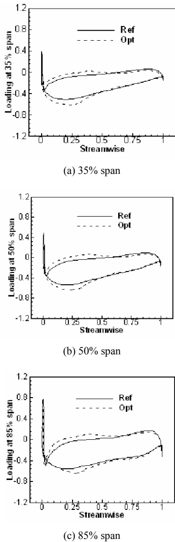
Fig. 8. Blade loading.
